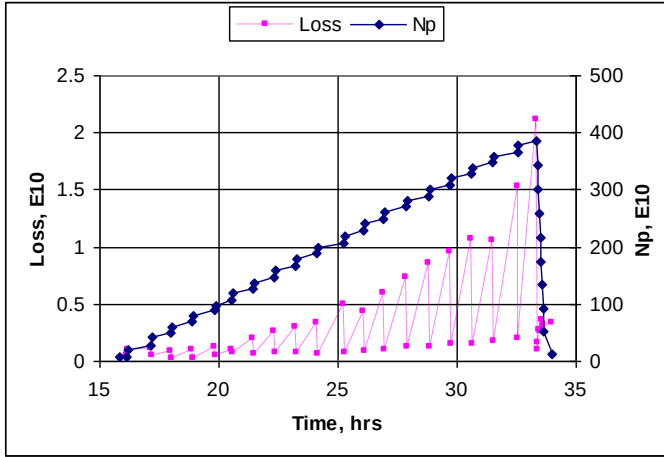
Figure 6: Antiproton beam intensity and losses over a stashing cycle. In blue diamonds are the numbers of antiprotons in the Recycler before and after injections/extractions. The pink squares represent beam losses during injections/extractions (lower value data points) and between injections (higher value data points).
