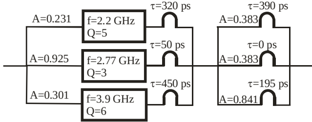
Figure 3: Schematic of the stacktail prototype equalizer
