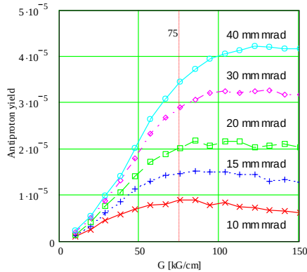
Figure 1: Simulated dependence of antiproton yield on the lithium lens gradient; rms proton beam size at the target is 130 \mu\text{m} , target length is 8 cm.
