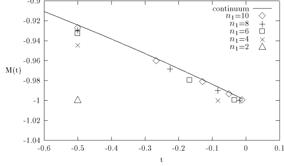
Figure 3: The behaviour of the amplitude M(t) for n_1 = 2, 4, 6, 8, 10 for small values of t .
