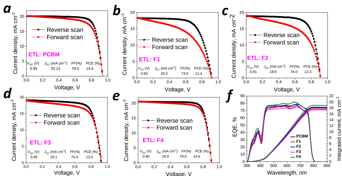
Figure 5 J - V curves measured in forward and reverse directions at a scan rate of 10 \text{ mV s}^{-1} for p-i-n perovskite solar cells assembled with different ETLs: PC 61 BM (a), F1 (b), F2 (c), F3 (d), F4 (e), and (f) EQE spectra of PSCs using different fullerene-based ETL materials.
