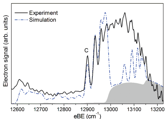
Figure 5. Experimental (solid line) and simulated (dashed line) \text{KrO}^- SEVI spectrum. Simulated spectrum is shifted by 10\text{ cm}^{-1} toward higher eBE to match the position of the origin (peak C). Shaded region represents the bound-free transition contribution to the simulated envelope.
