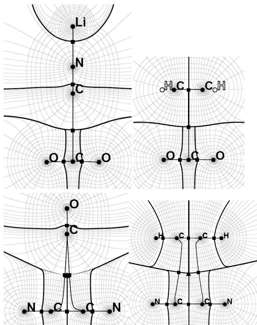
Figure 3. Electron density map of the CO 2 :NLi, CO 2 :C 2 H 4 , NCCN:CO, and NCCH:HCCH complexes obtained at the M05-2x/6-311++G(d,p) computational level. The circles, squares, and triangles represent the position of the atoms, bond, and ring critical points, respectively. The bond paths are shown.
