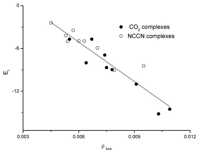
Figure 4. E_i per interaction (kJ mol -1 ) vs \rho_{\text{bcp}} (au). The adjusted linear correlation presents a square correlation coefficient of 0.87.
