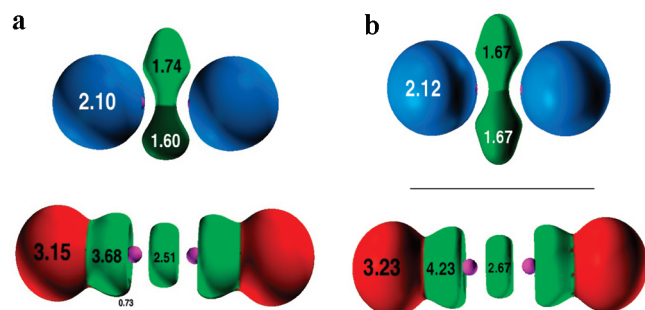
Figure 7. ELF isosurface representation for (a) compound NCCN: \text{H}_2\text{CCH}_2 and (b) the isolated monomers.
